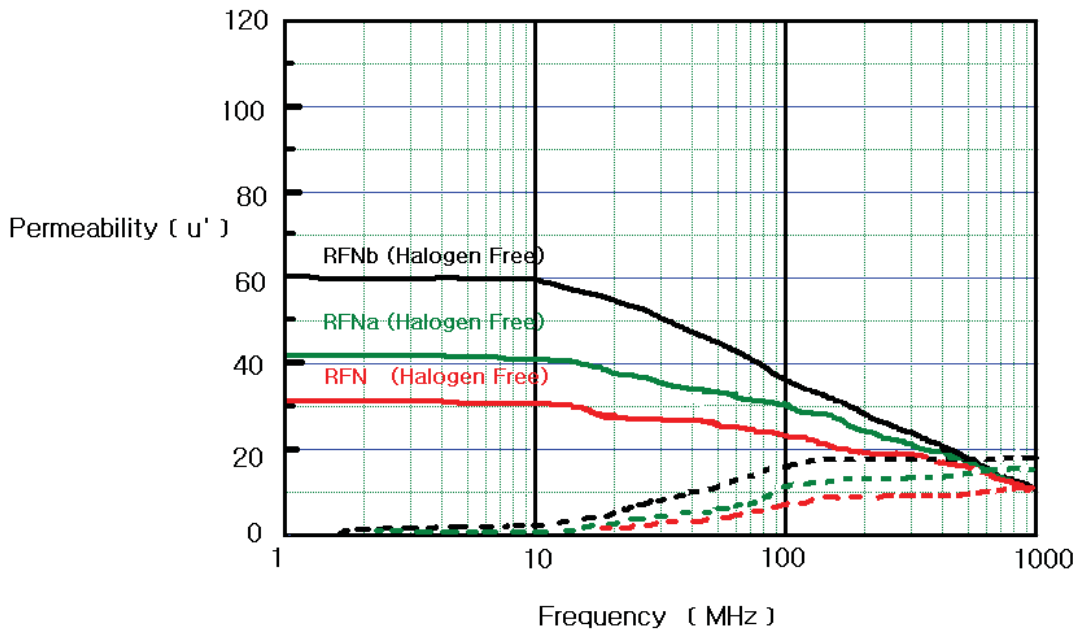
Permeability of EMI Absorber
